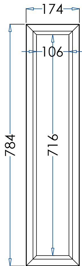
[ Front ]
